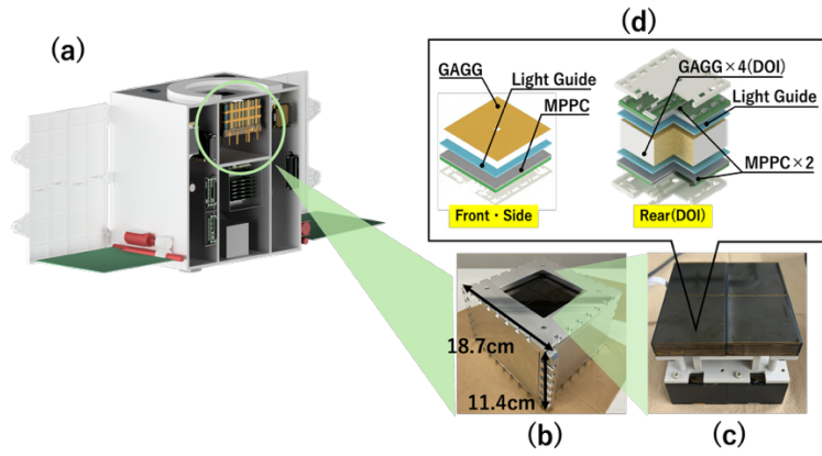
Figure 1. (a) overview of the GRAPHIUM (b) overview of the INSPIRE (c) Hybrid Compton camera part (d) Configuration of each sensor unit
