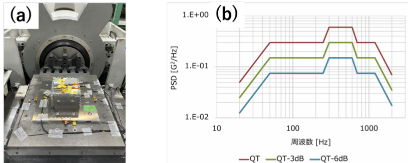
Figure 4. (a) set up of engineering model vibration test, (b) Power spectral density (PSD) in QT
