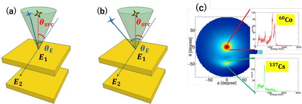
Figure 3. Schematic view of ARM cut. (a) source-like events (b) background events (c) Energy spectra extracted from selected regions in the image reconstructed with the ARM cut
