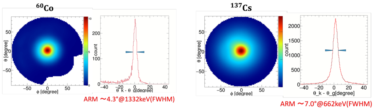
Figure 2. left: Co-60 image using engineering model, right: Cs-137 image using engineering model
