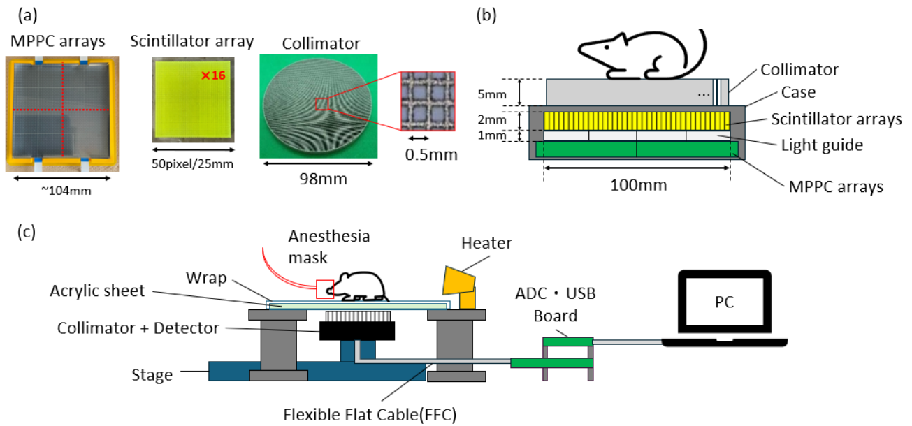
Fig. 1 (a) Photographs of the MPPC arrays, scintillator arrays, and tungsten collimator used for the detector. (b) Configuration of the detector. (c) Schematic diagram of the imaging setup.
