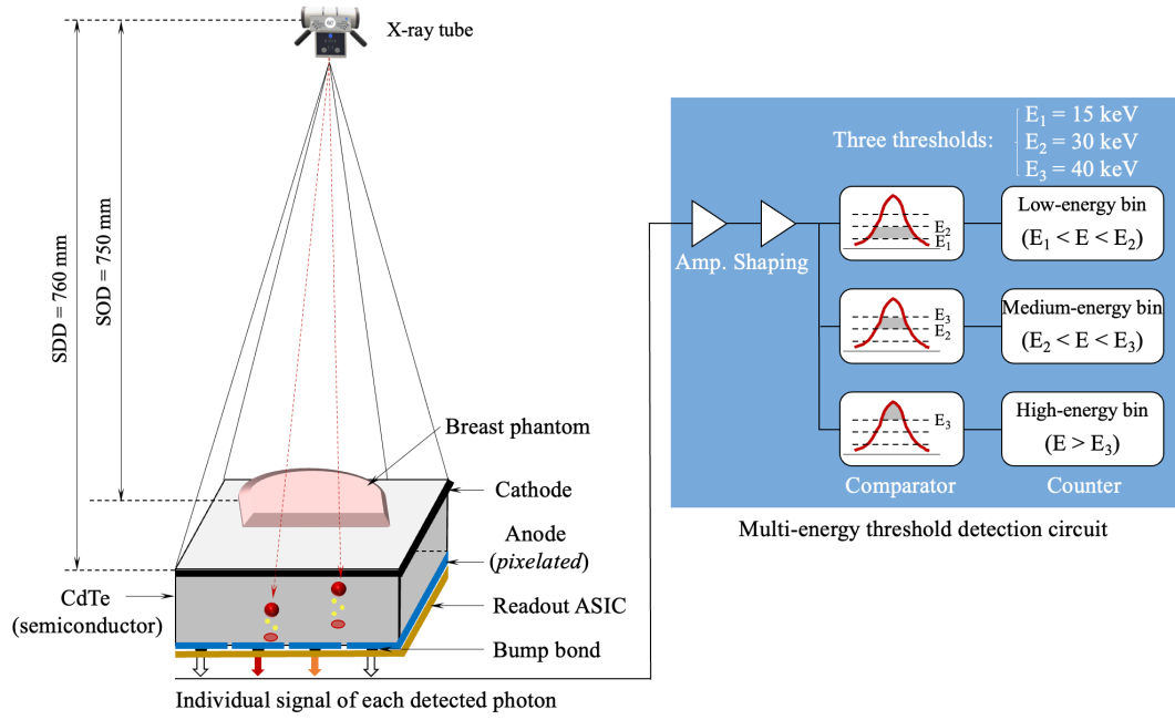
Figure 1. Schematic diagram of the CdTe-based photon-counting detector system for breast phantom imaging with three energy thresholds
